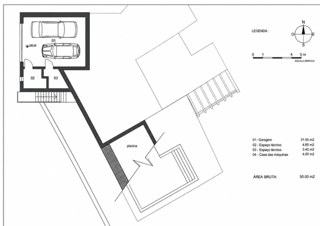
Basement Plan
